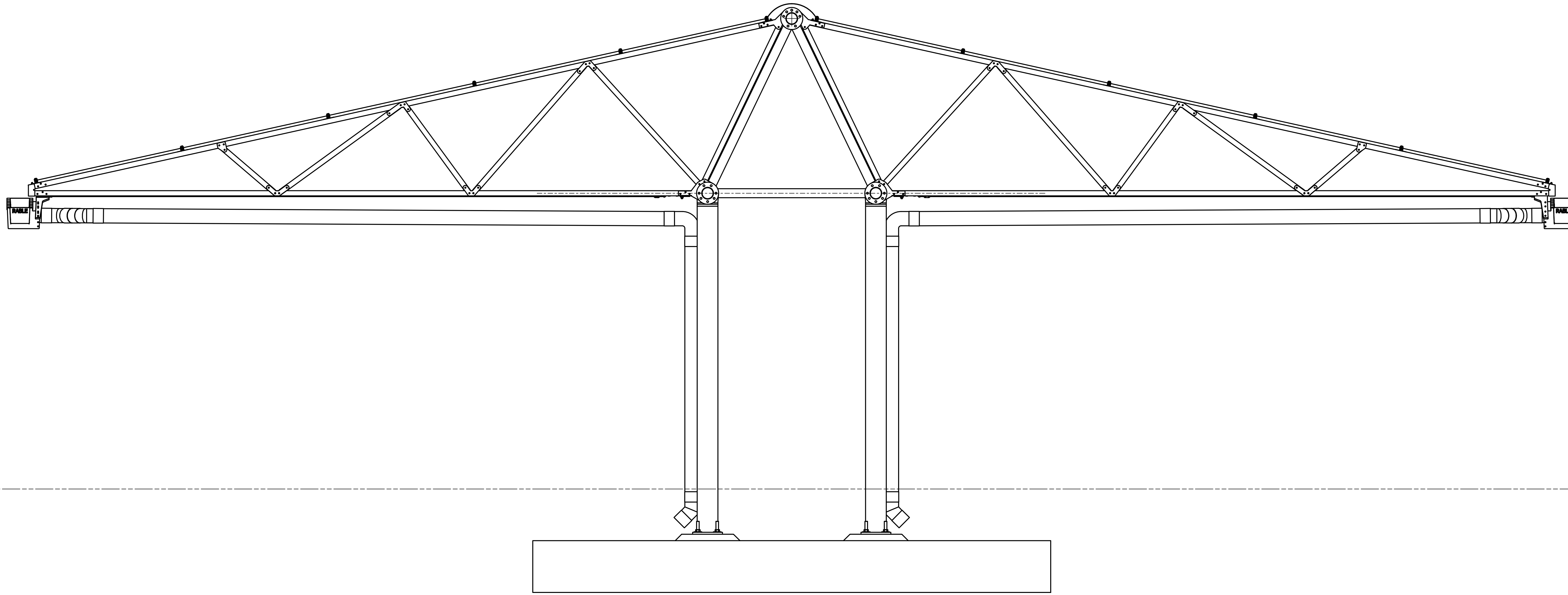
Frontview Standard Module with gutters & drainage
